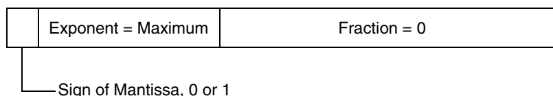
Figure 1-21. Infinity Format
