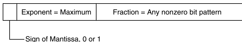
Figure 1-22. Not-a-Number Format
