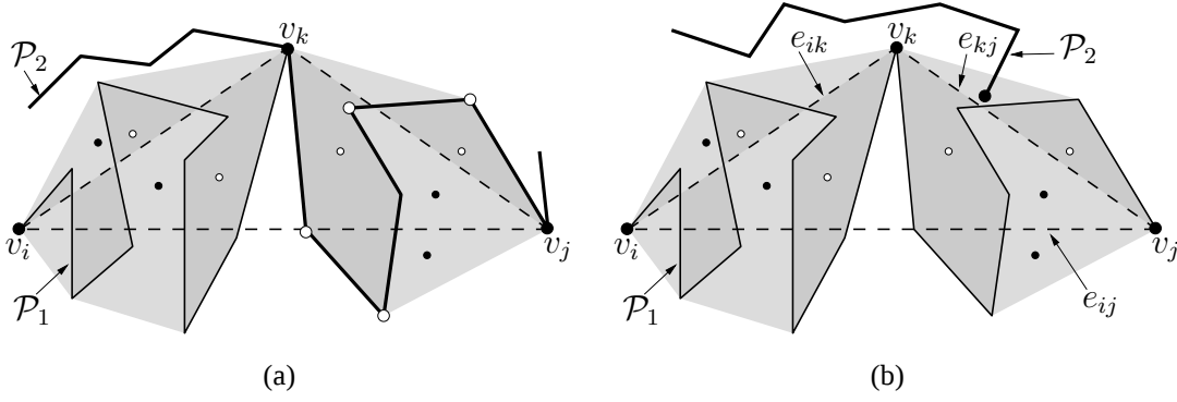
Figure 9. Update of the arrangement of the features after the insertion of a vertex v_k in (a) the coincidence case, and (b) the incidence case.
