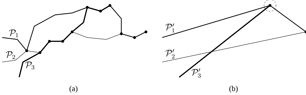
Figure 7. (a) Partially coincident polylines \mathcal{P}_1 , \mathcal{P}_2 , and \mathcal{P}_3 ; and (b) their topologically inconsistent outcomes from our simplification \mathcal{P}'_1 , \mathcal{P}'_2 , and \mathcal{P}'_3 .
