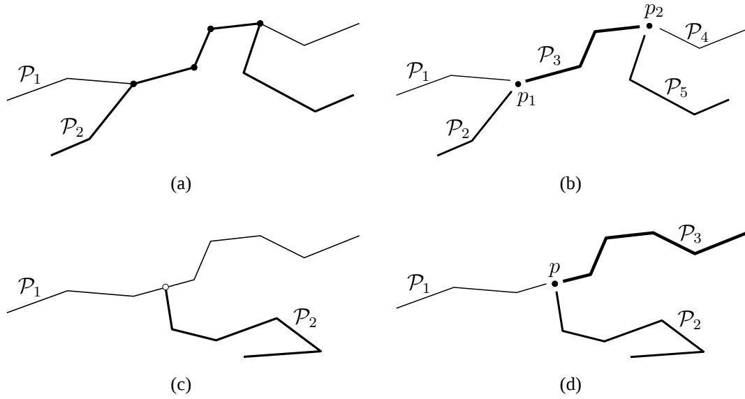
Figure 2. Geometrical redundancies and their respective correct topological representations: (a) the partially coincident polylines P_1 and P_2 , and (b) their partitioning into the disjunct subsets P_1 , P_2 , P_3 , P_4 , P_5 , p_1 , and p_2 ; (c) the incident polylines P_1 and P_2 , and (d) their partitioning into the disjunct subsets P_1 , P_2 , P_3 , and p .
