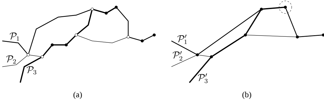
Figure 8. (a) Polyline P_1 , P_2 , and P_3 with their essential vertices; and (b) their topologically consistent outcomes from the modified version of Saalfeld's simplification P'_1 , P'_2 , and P'_3 .
